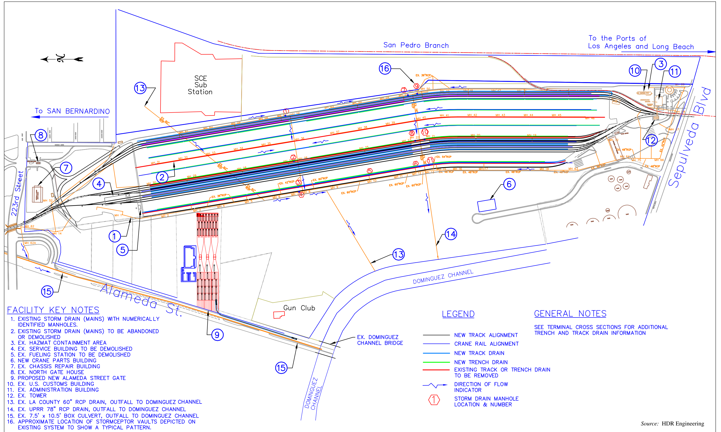
Figure 8. UP ICTF Storm Drain Plan
