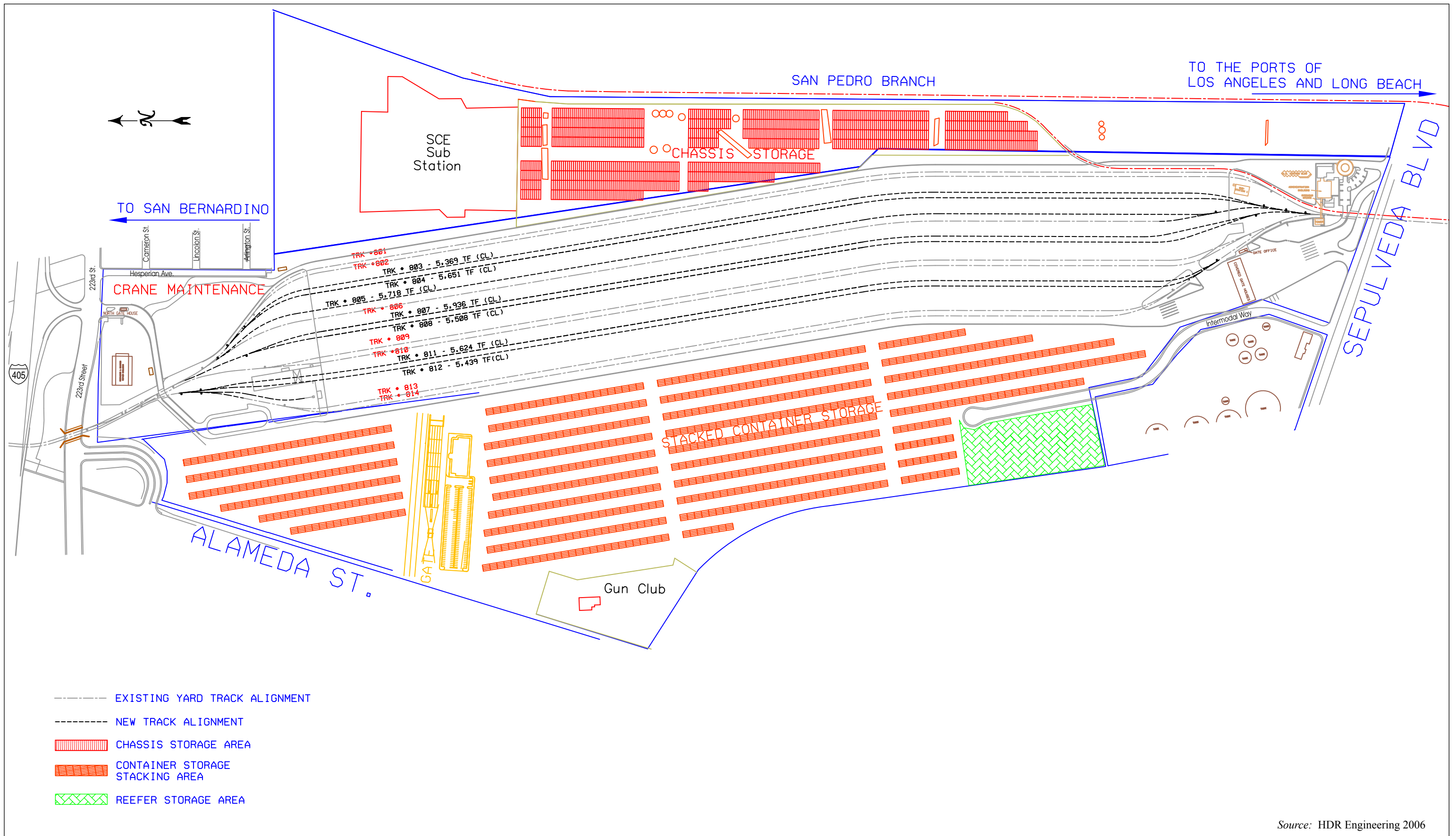
Figure 20. UP ICTF RTG Crane Alternative
