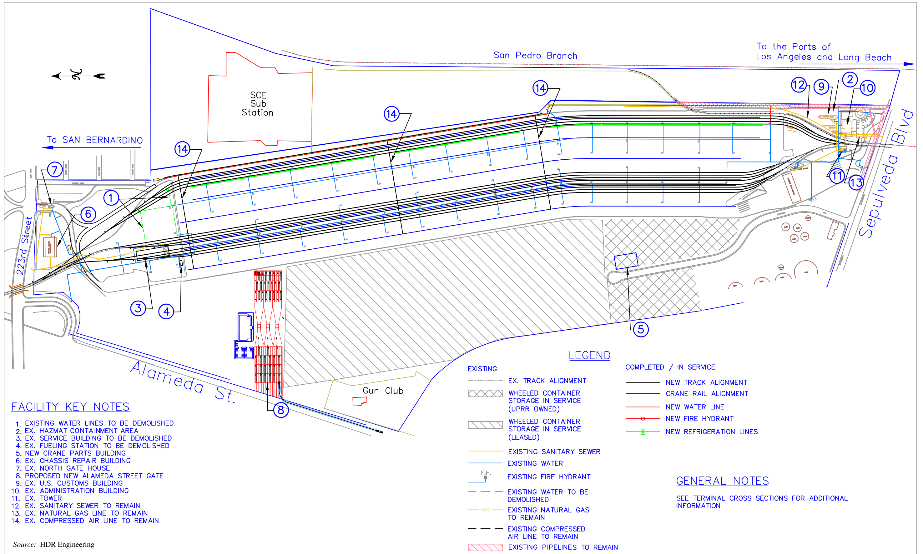
Figure 10. UP ICTF Water, Sewer and Pressurized Air Plan
